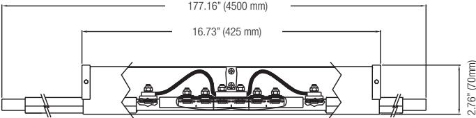
Expansion Section (Typical)
